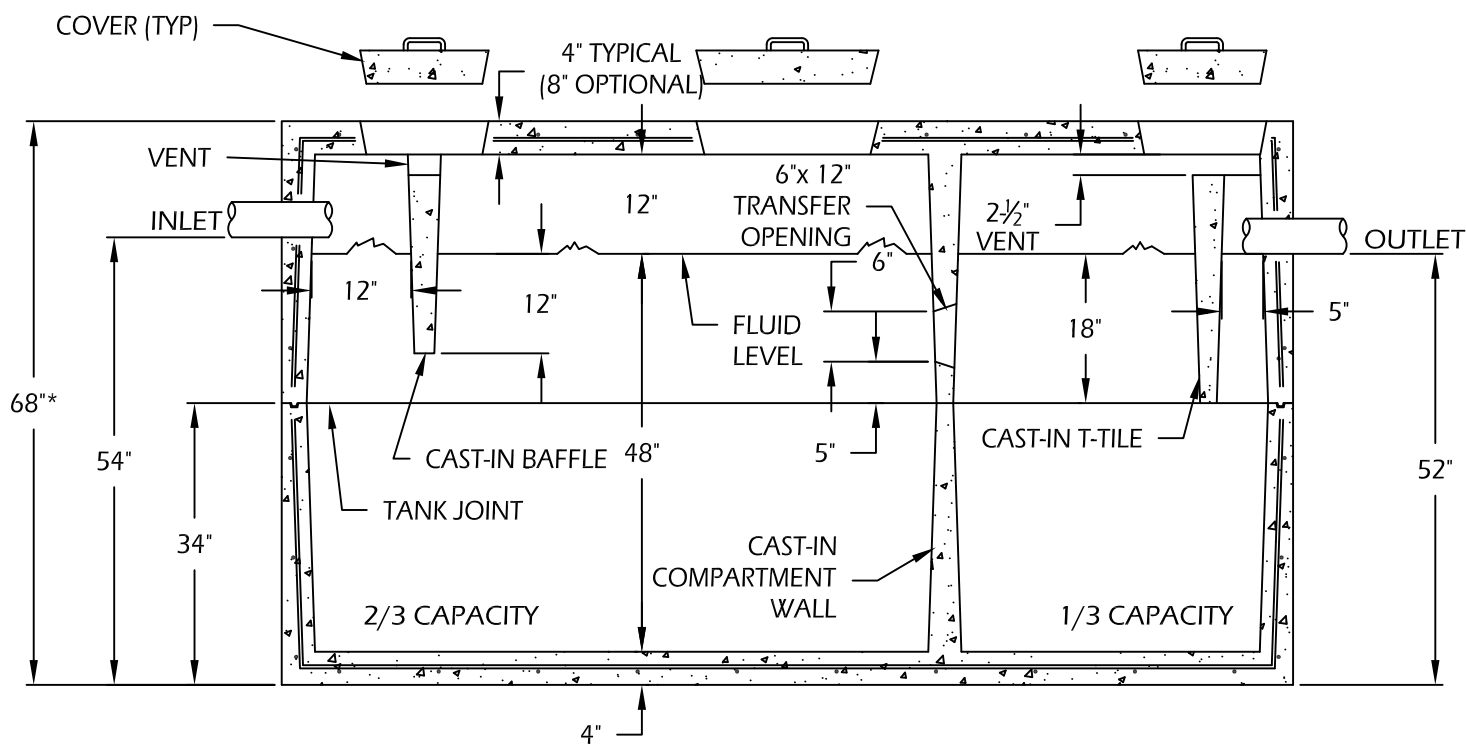
SECTION VIEW
