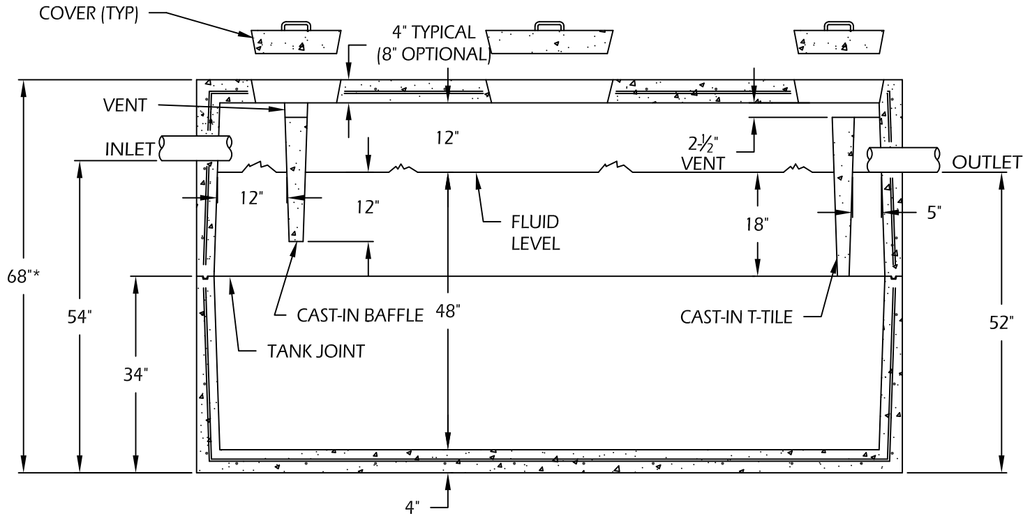
SECTION VIEW
