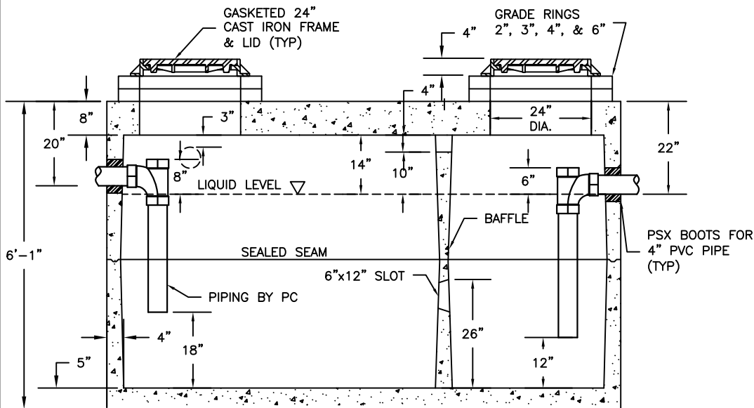
SECTION VIEW
