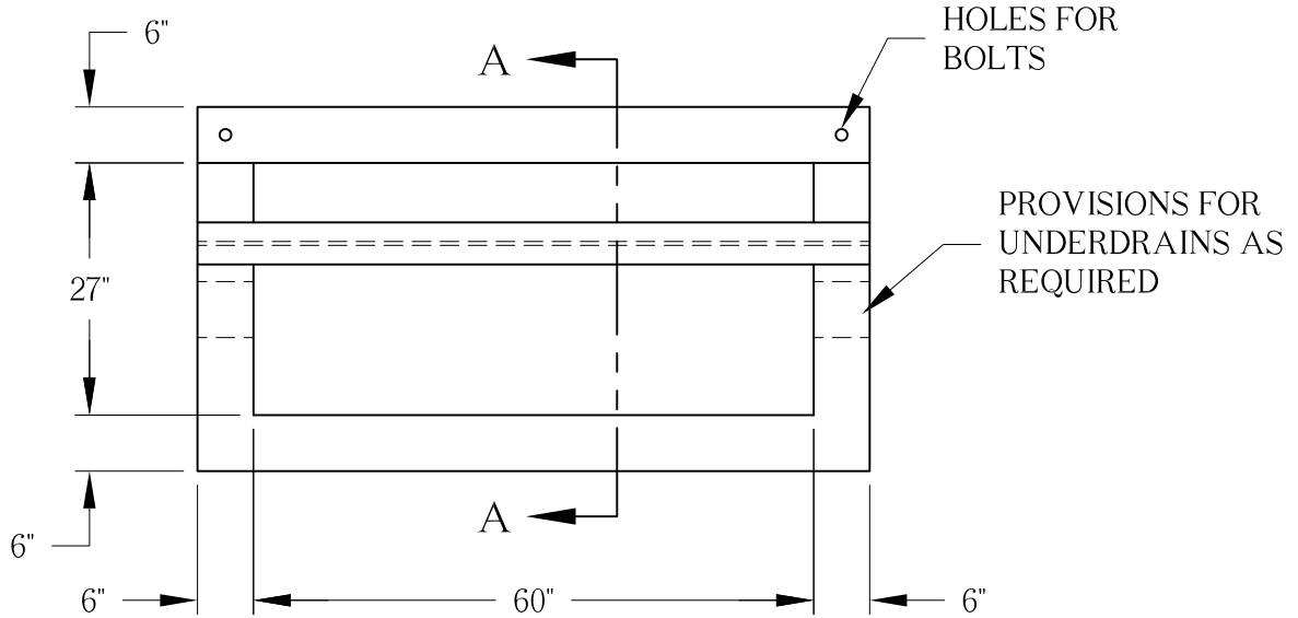
TOP VIEW
