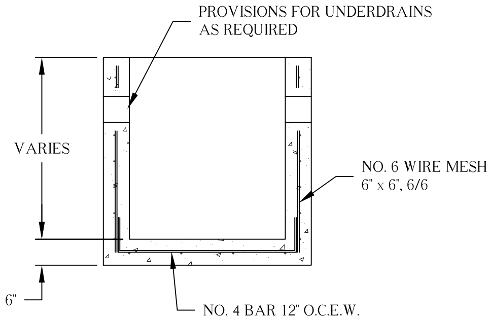
SECTION VIEW
