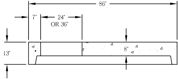
FLAT SLAB TOP
