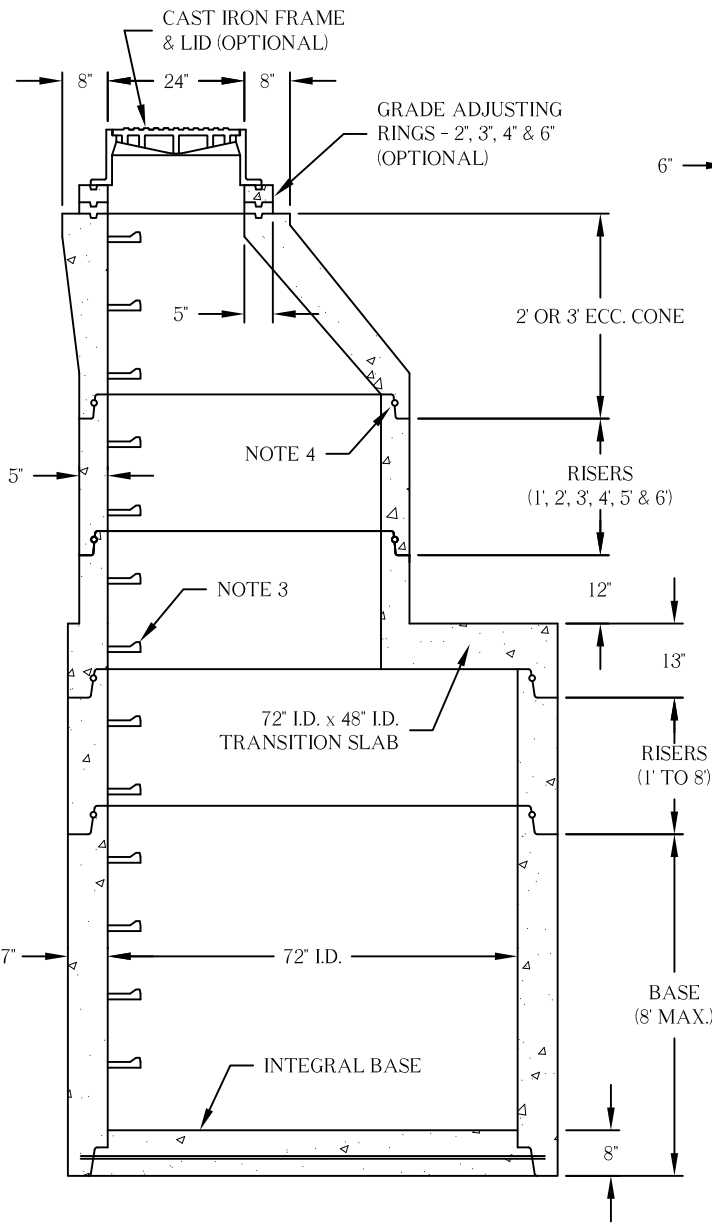
SECTION VIEW
