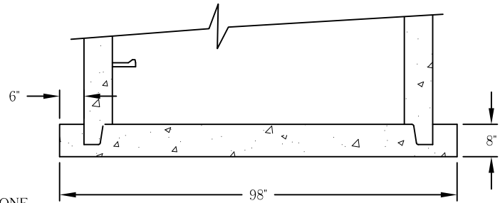
ALTERNATE EMBEDDED BASE
