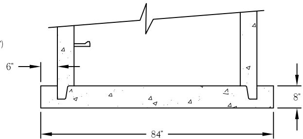
ALTERNATE EMBEDDED BASE
