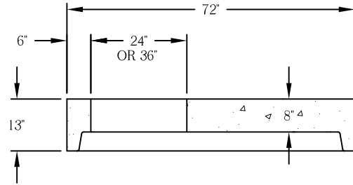
FLAT SLAB TOP
